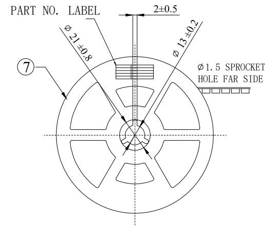
STYLE AND DIMENSION OF REEL
